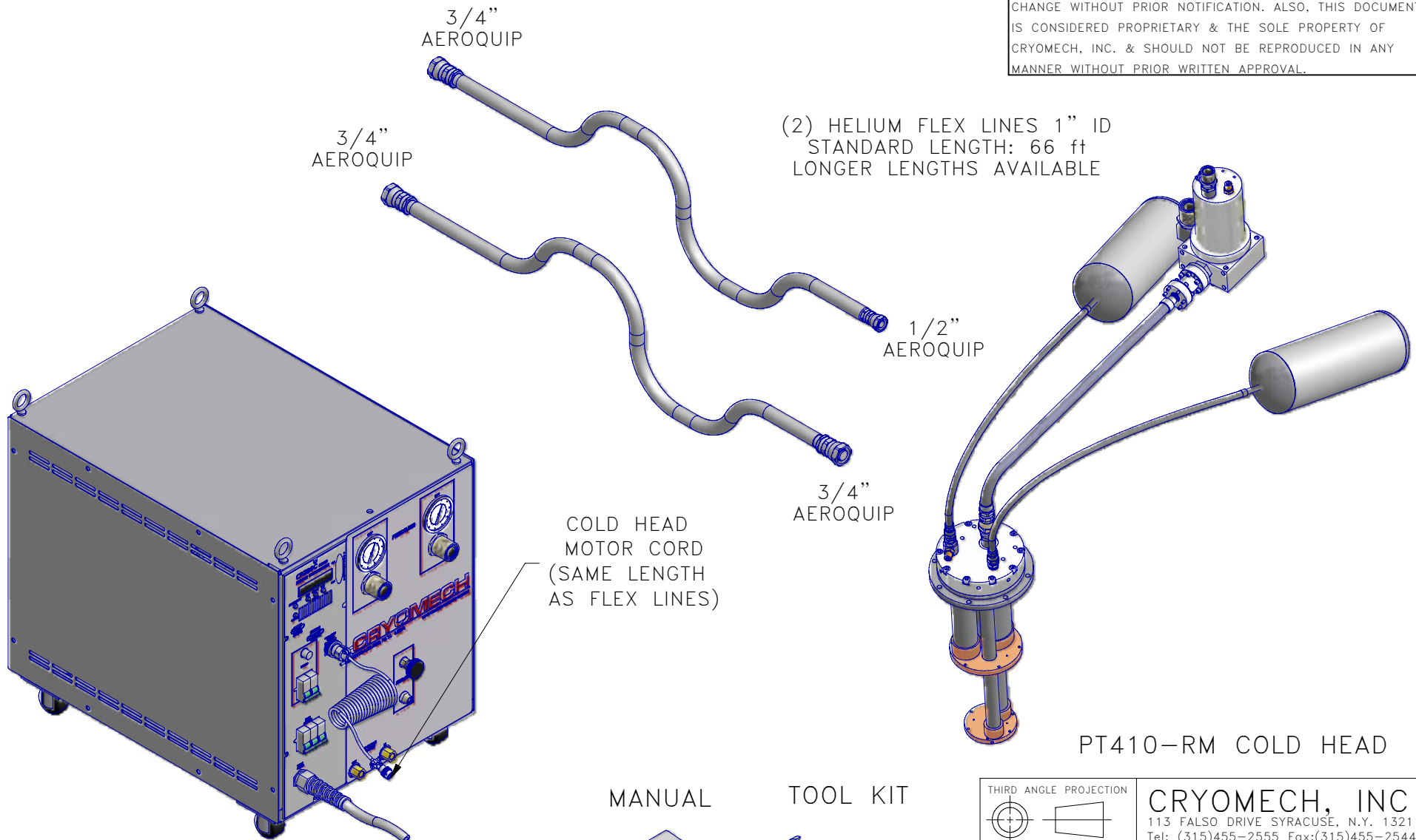
CP289C COMPRESSOR PACKAGE (WATER COOLED)
